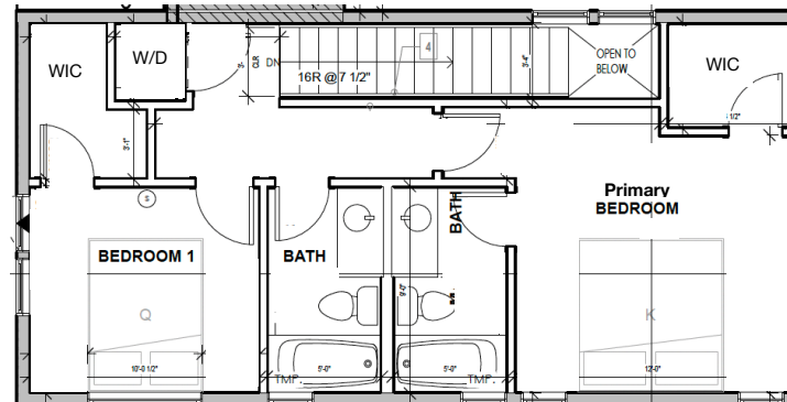
Second Floor
